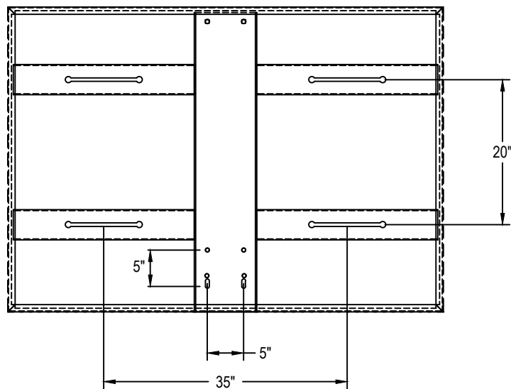
REAR
